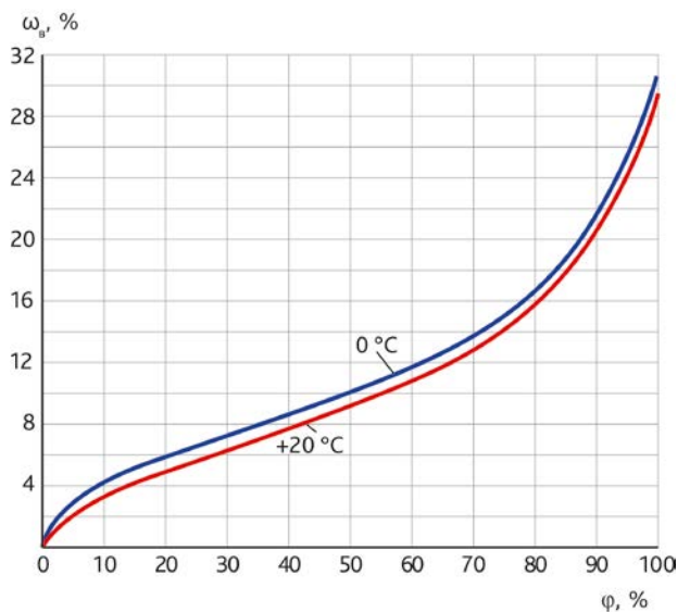
Figure 1. Water vapor sorption isotherm for wood.
