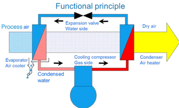
Figure 1. Functional diagram of the condensation method.
