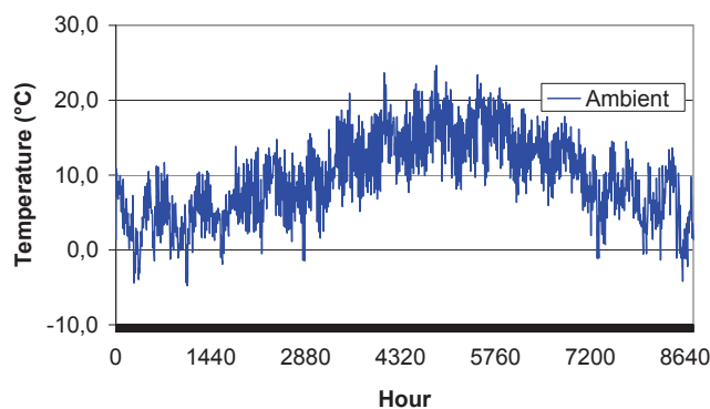
Figure 3. Ambient temperature TRY record Cardiff (Wales, UK).
