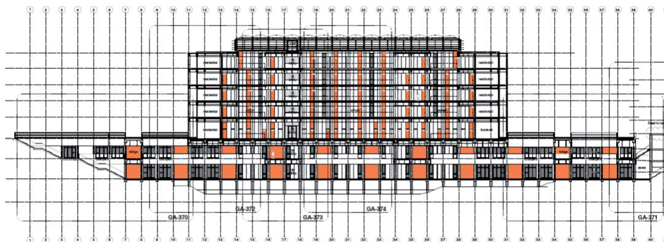
Figure 2. Vertical (side) view of the development.
