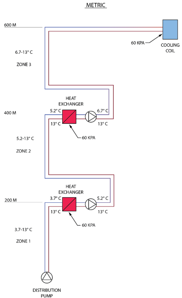
Figure 5. A diagram of a chilled water distribution system for a 600m building where the distribution is split into three parts to regulate static pressure.
